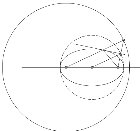
Fig.1. Composition of Tangent on Ellipse
