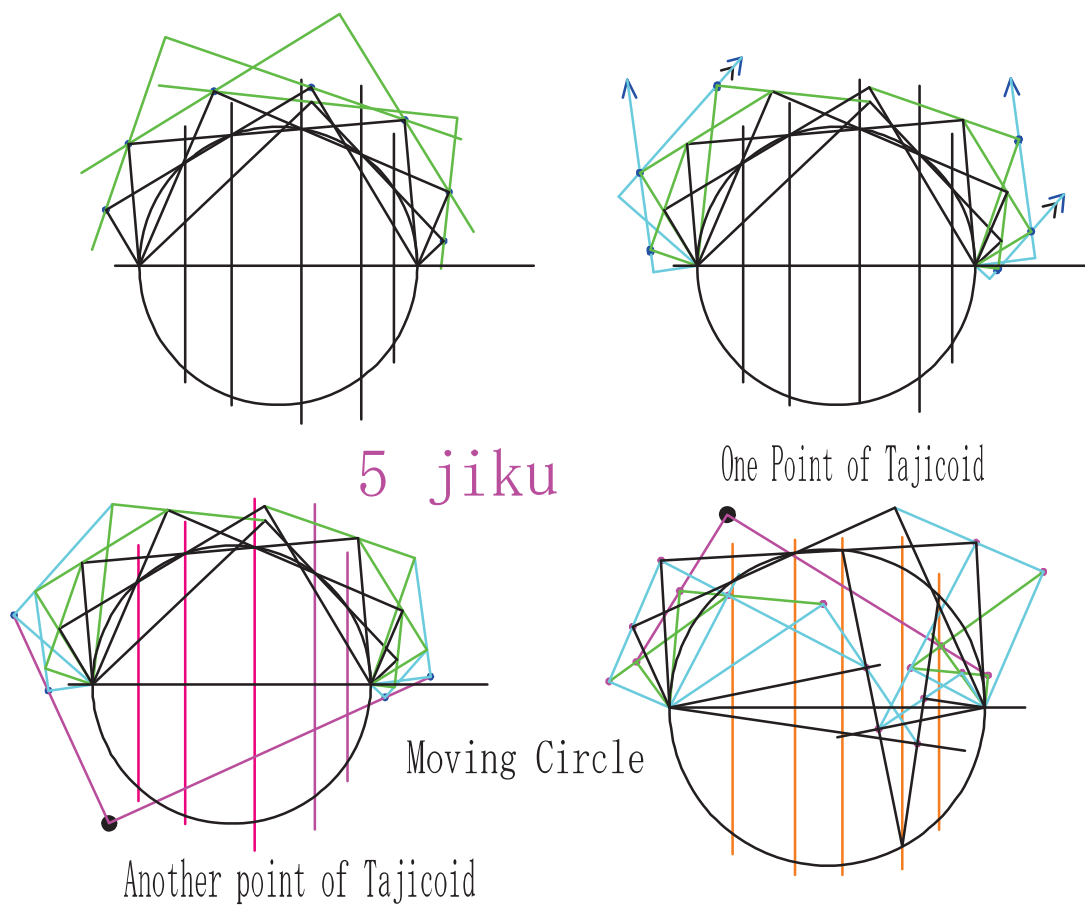
Fig.11. Def. Figure of Tajicoid
