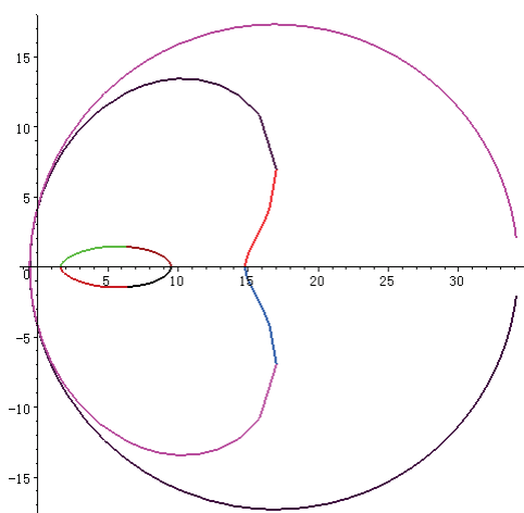
Fig.1. Composition of Tangent on Ellipse
