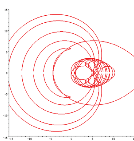
Fig.2. Oval extended from Ellipse
