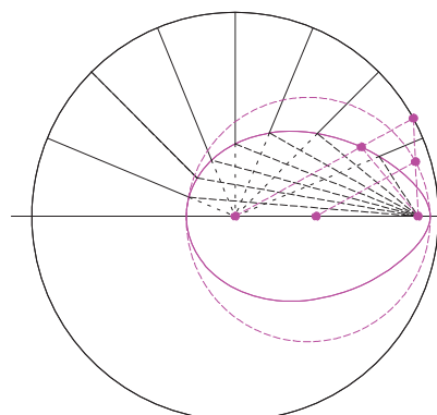
Fig.2. Oval extended from Ellipse
